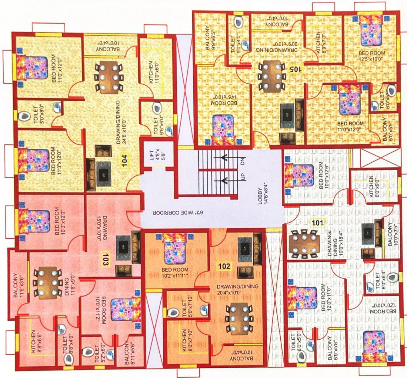
TYPICAL GROUND TO FOURTH FLOOR PLAN BLOCK - B
