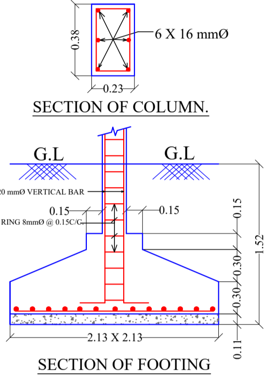
SECTION OF FOOTING
