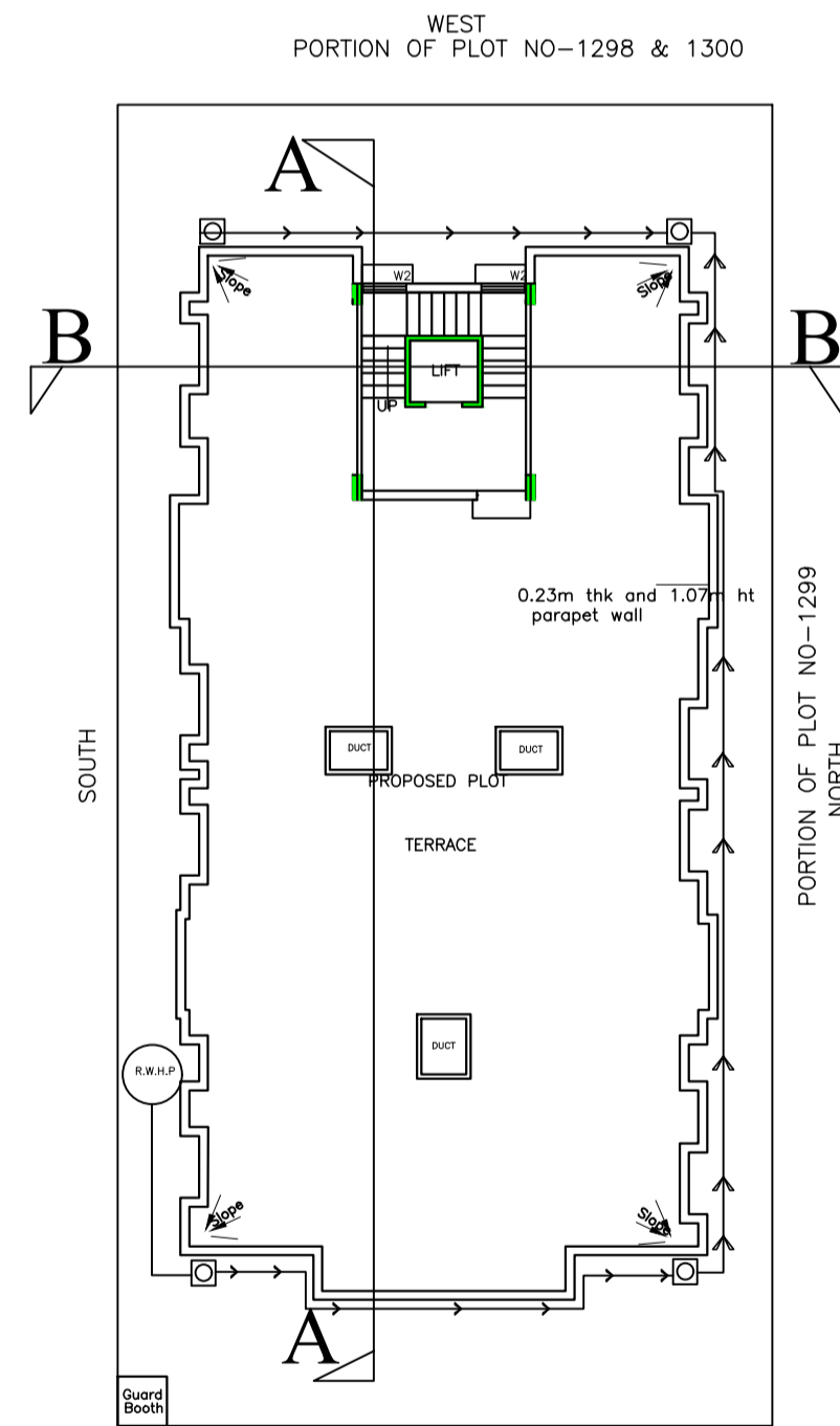
RAIN WATER HARVESTING PLAN
