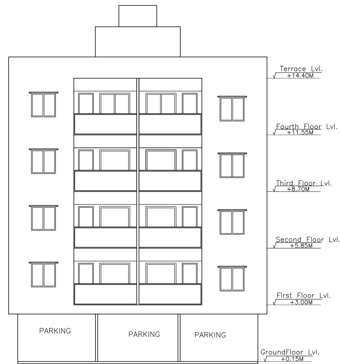
FRONT ELEVATION
