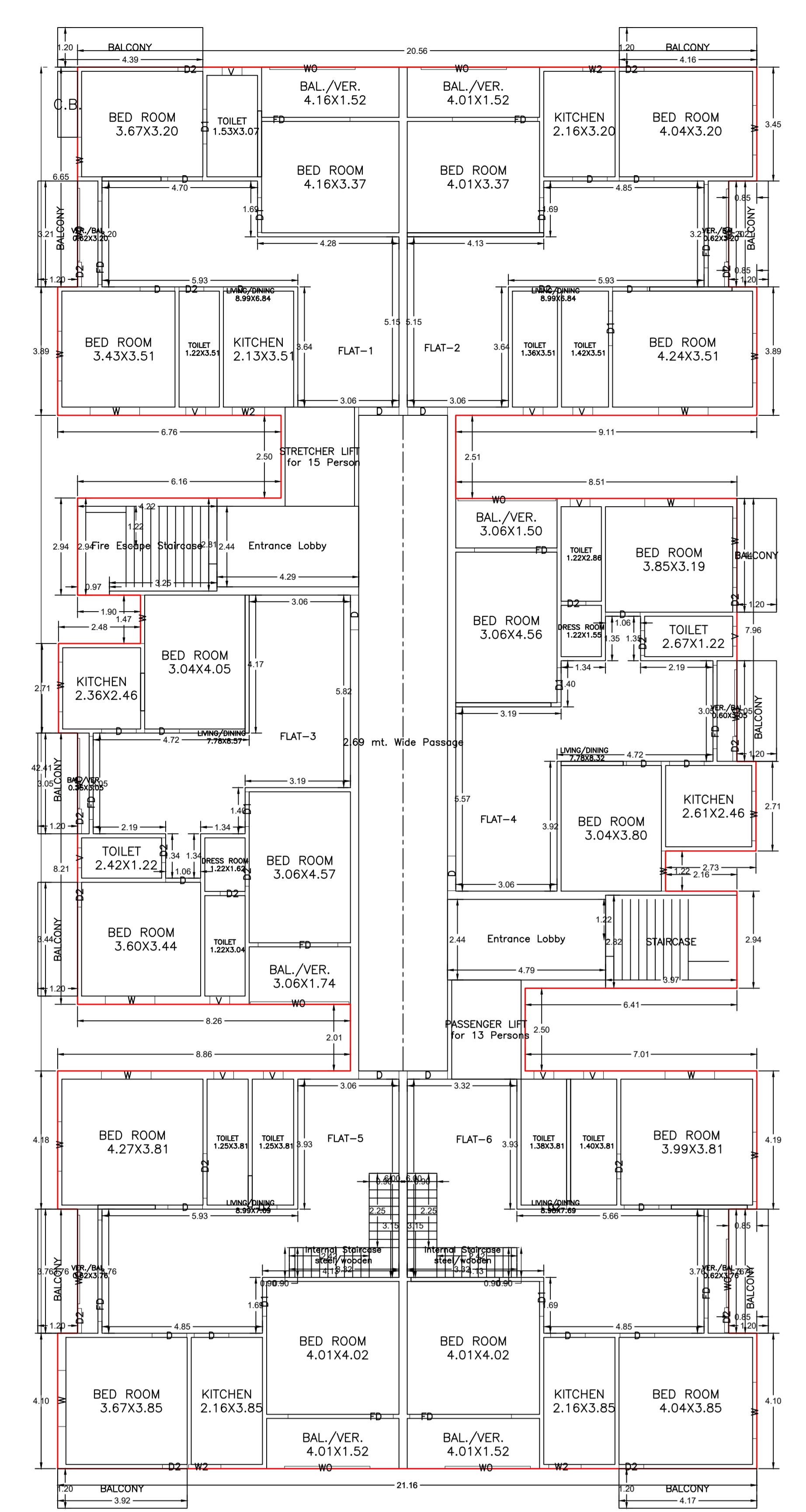
SIXTH FLOOR PLAN (Proposed) (SCALE: 1:100)
