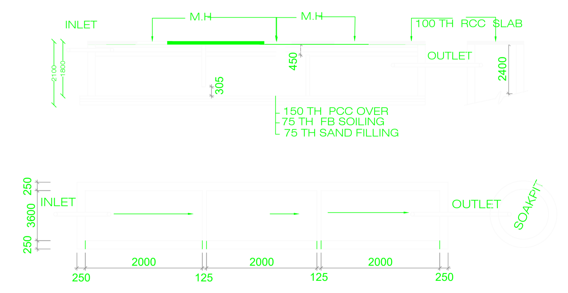
DETAIL OF SEPTIC TANK (SCALE=1:100)
