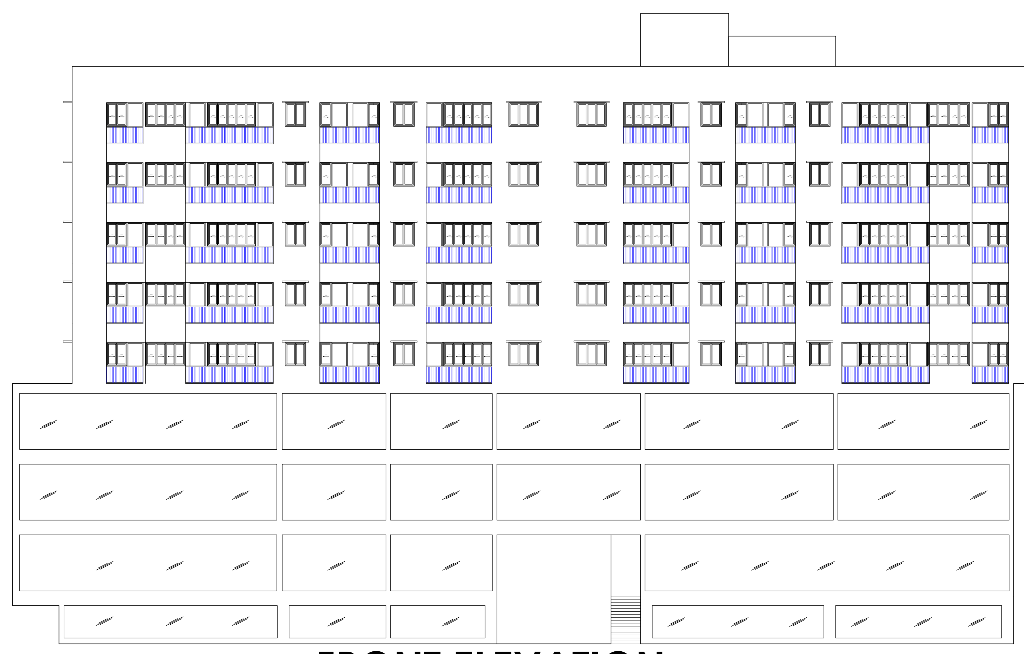
FRONT ELEVATION
