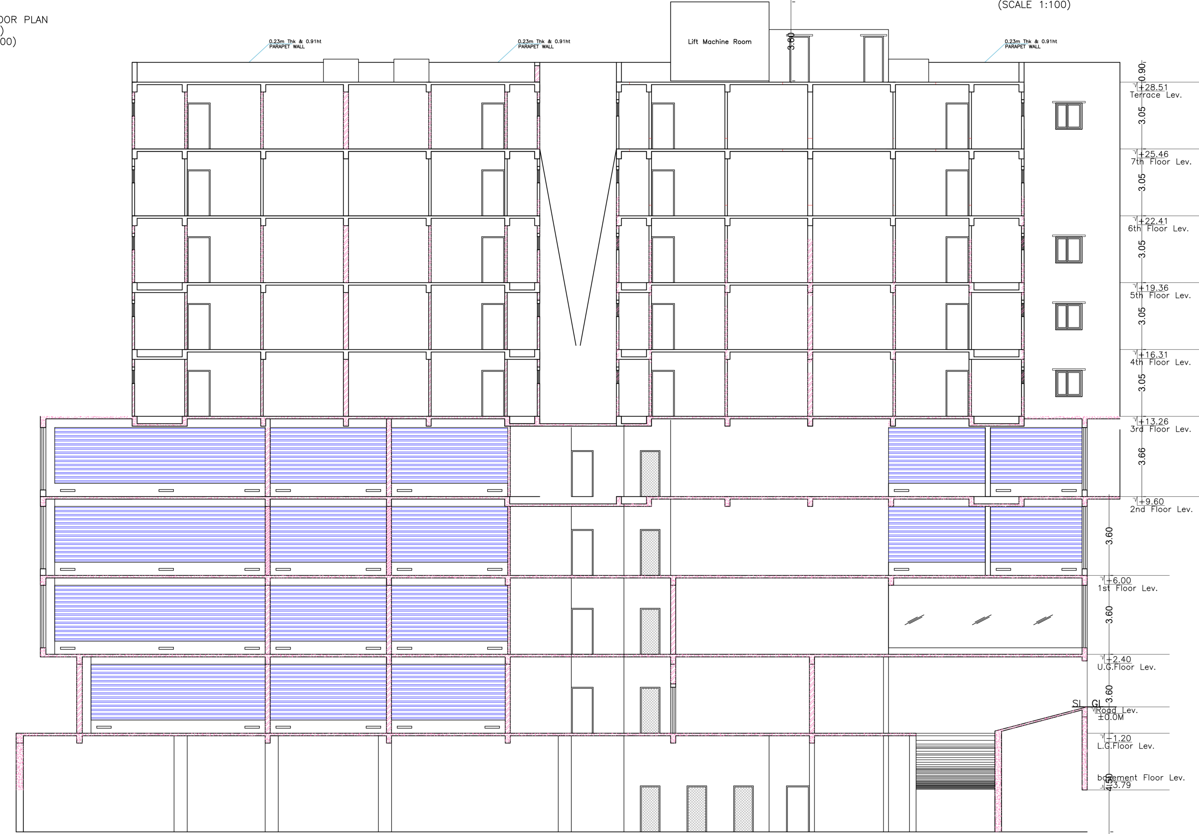
SECTION AT -XX
