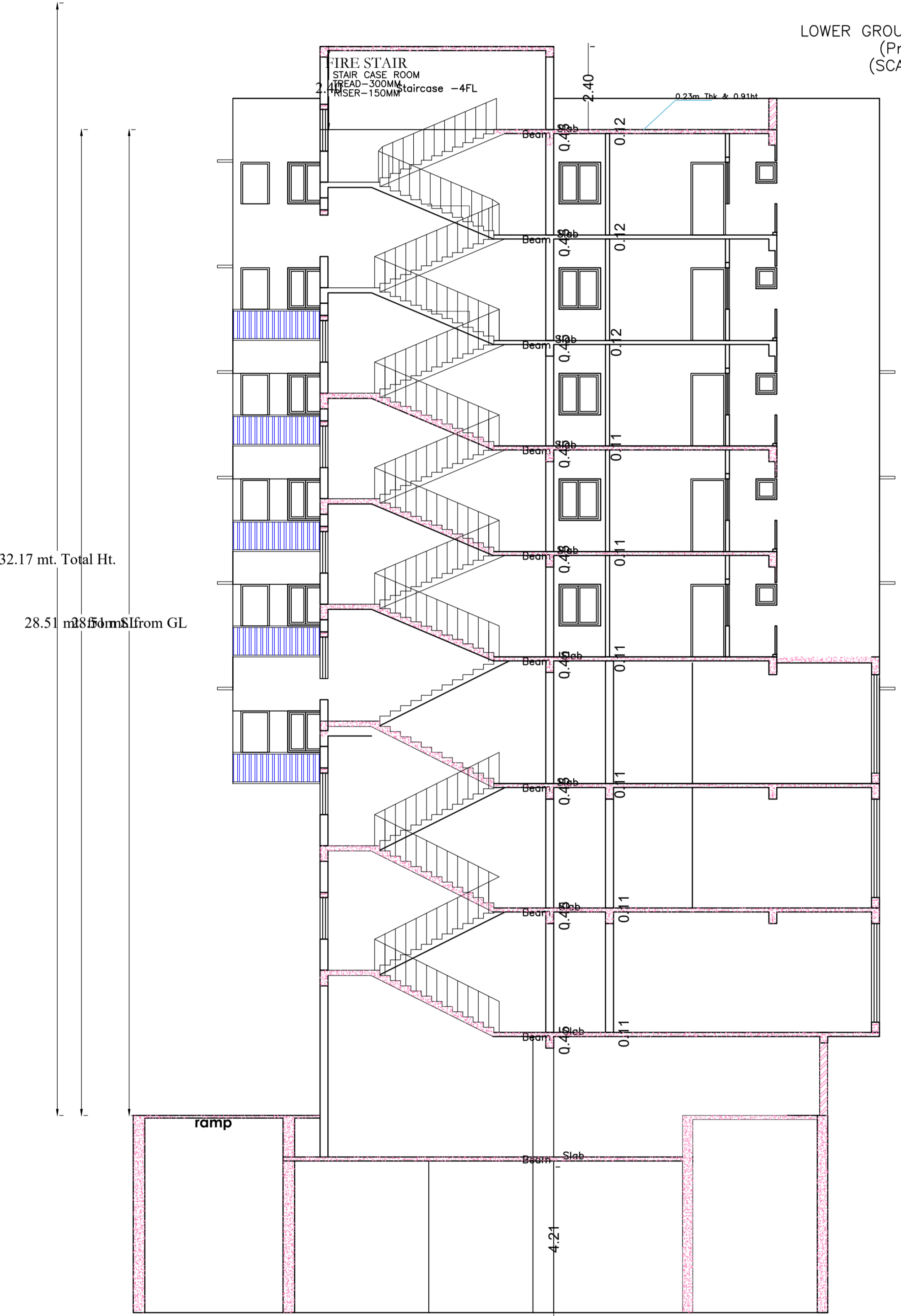
SECTION AT YY
