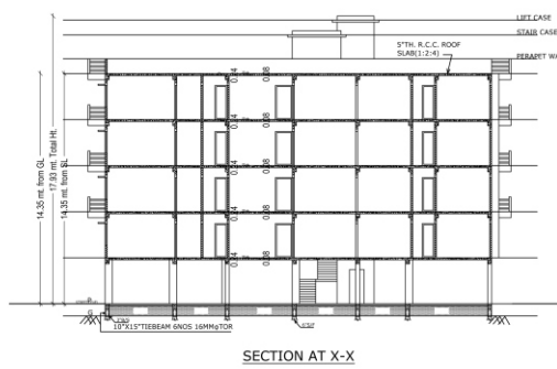
SECTION AT X-X
