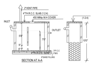
SECTION AT A-A
