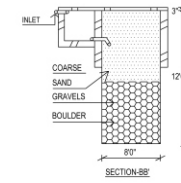
RAIN WATER HARVESTING SCHEME
