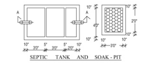
SEPTIC TANK AND SOAK - PIT
