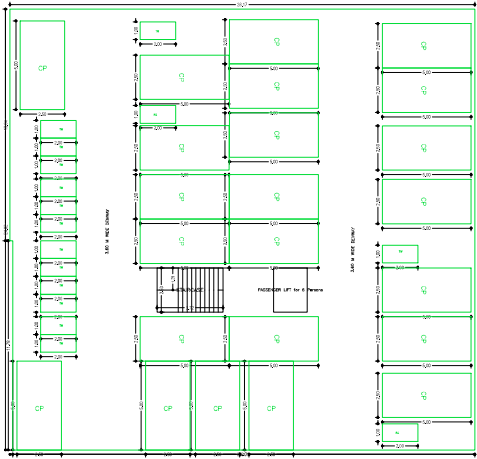
BASEMENT FLOOR PLAN (SCALE: 1:100)
