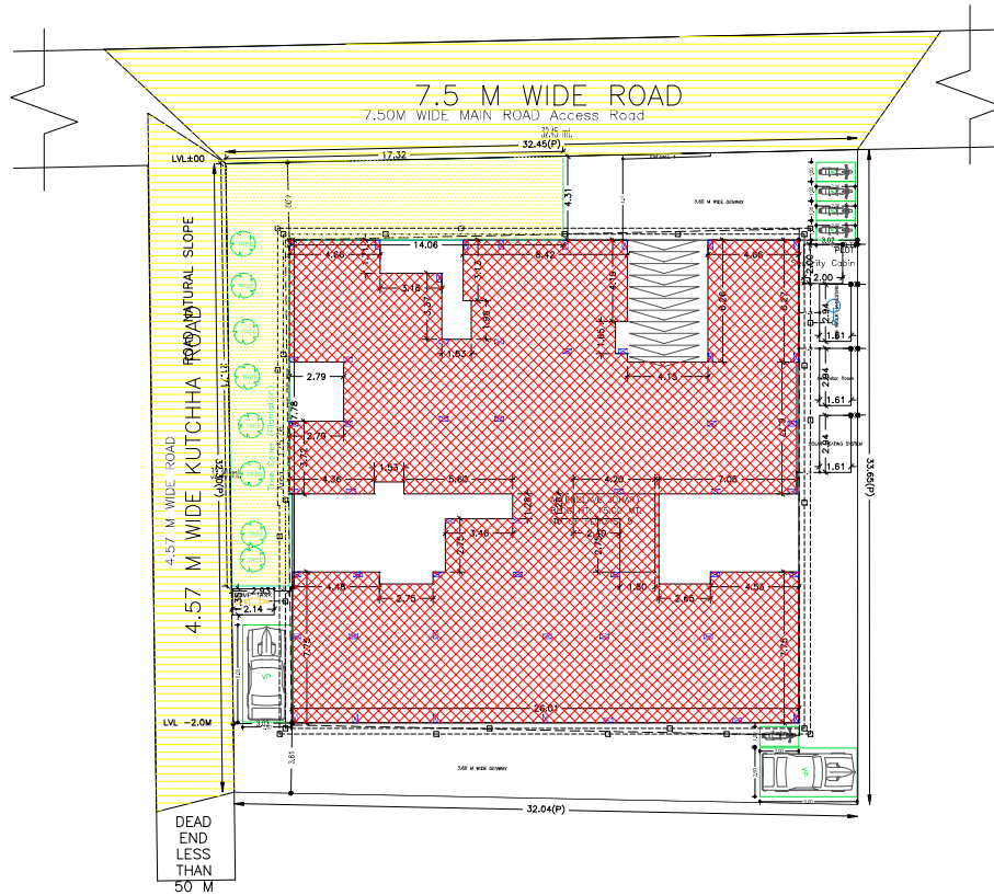
SITE PLAN
