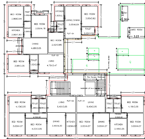
GROUND FLOOR PLAN (Proposed) (SCALE: 1:100)
