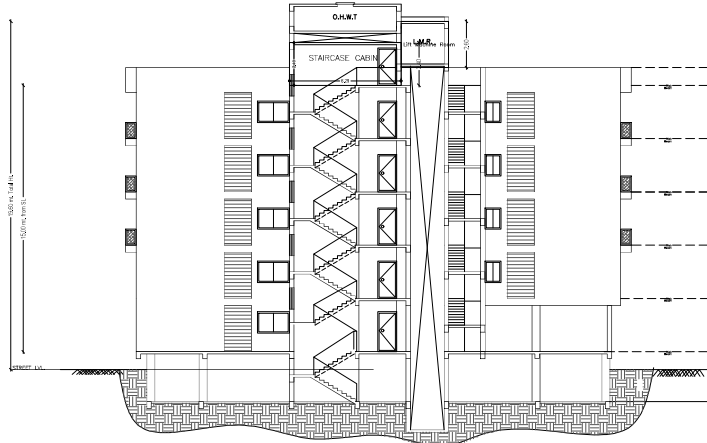
SECTION - XX'
