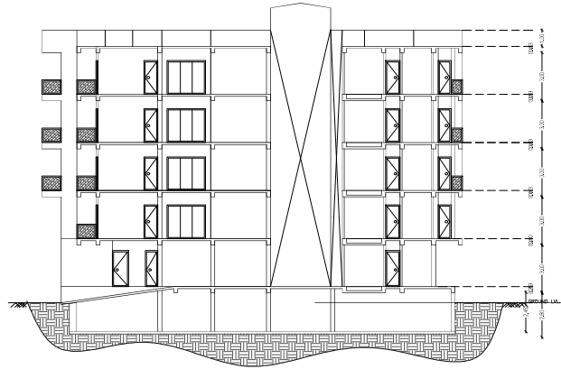
SECTION - YY'
